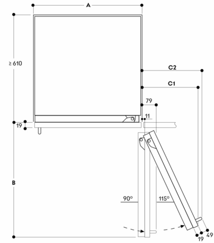
Wandabstand RVB/RVC/RVF/RVW
